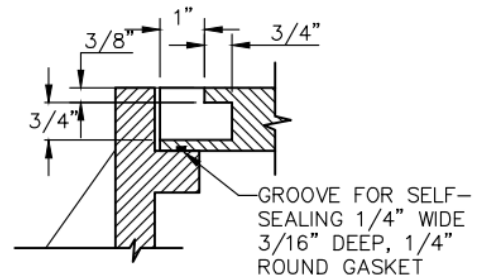
PICK HOLE SELF-SEALING GROOVE
