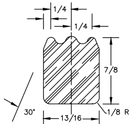
TYP. CROSS SECTION ON ALL STEPS
