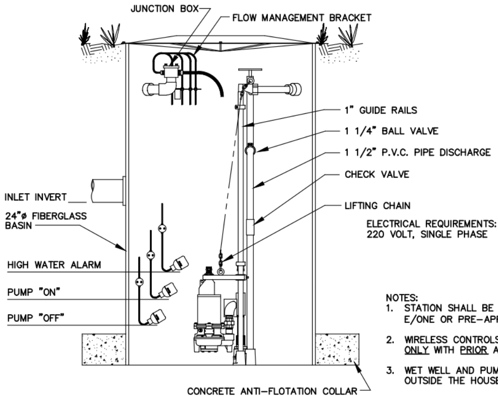
BASIN ASSEMBLY SIDE VIEW
