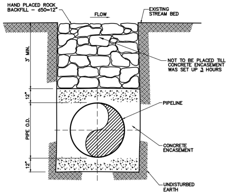
SECTION E - E ENCASEMENT AND BACKFILL DETAIL
