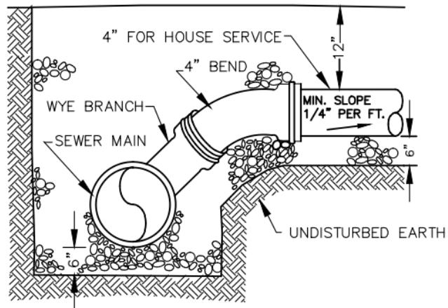
TYPICAL CONNECTION TO SEWER MAIN
